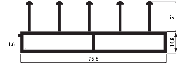
BT - A - 1,580 kg/m
