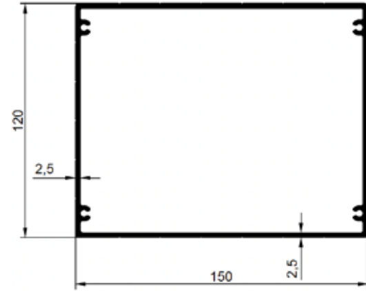
0132 3,789 Kg/m 150X120 DİREK
