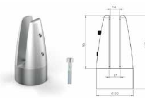
■ 500-605 Small Glass Holder
