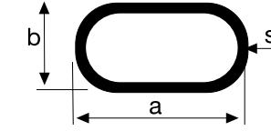
OVAL KUTU PROFİLLERİ Oval Box Profiles
