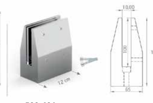
■ 500-604 Block Type Glass Holder (12cm)
