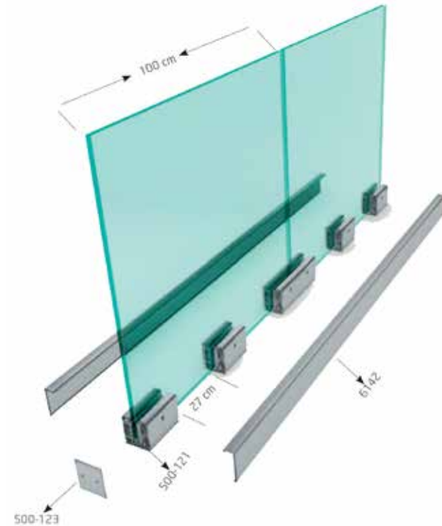
500-121 Glass Base Set-15 Cm
