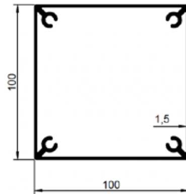
0094 2,253 Kg/m 100X100 DİREK
