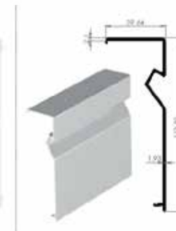
6150 Cover Profile With Led Channel (6 meters)
