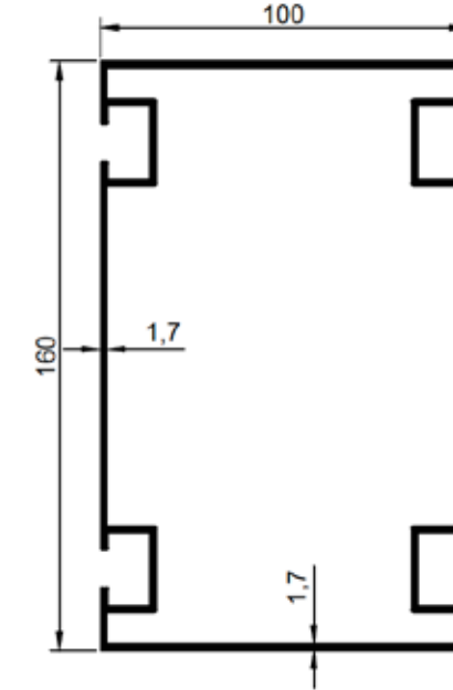
0128 3,245 Kg/m 160X100 DİREK
