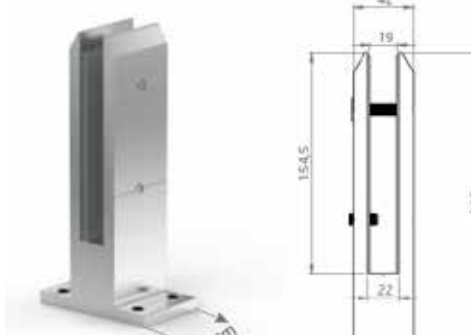
■ 500-602 Square Glass Holder
