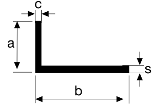
L KÖŞEBENT PROFİLLERİ 50×50 5 mm L Angle Trim Profiles
