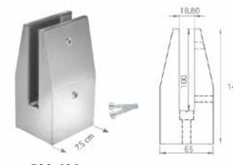
■ 500-606 Block Type Glass Holder (7,5cm)
