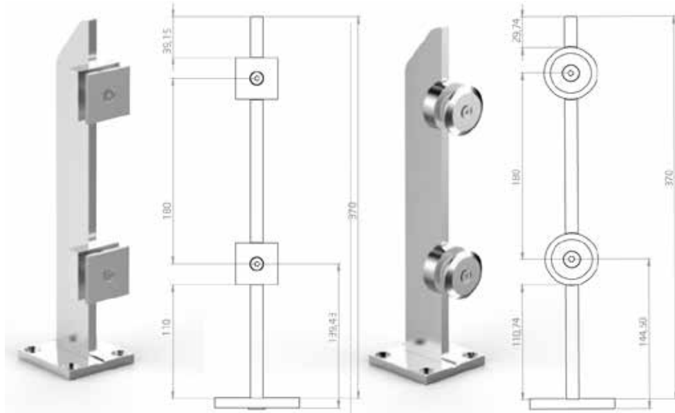
■ 500-610 Double Glass Connector With Lama Pilar - Square
