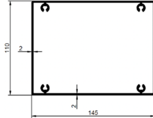
0166 3,249 Kg/m 110X145 DİREK
